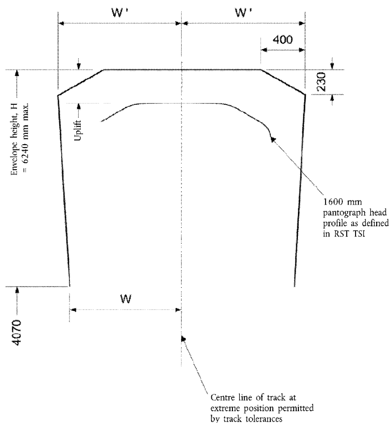
Figure 7.5.2.7 Pantograph gauge
